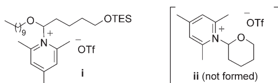
Figure 2. Possible cationic intermediates.
