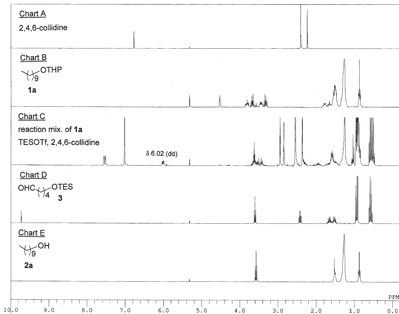
Figure 1. ^1\text{H} NMR charts for the reaction of 1a with TESOTf–2,4,6-collidine in \text{CD}_2\text{Cl}_2 .
