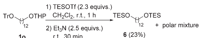
Scheme 5. Direct conversion of THP ether into TES ether.
