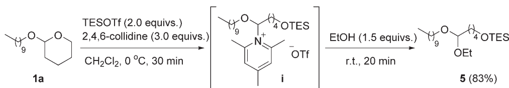
Scheme 4. Trapping of the intermediate with EtOH.
