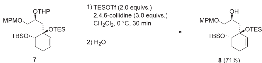
Scheme 6. Chemoselective deprotection of THP ether 7 in the presence of many functional groups.
