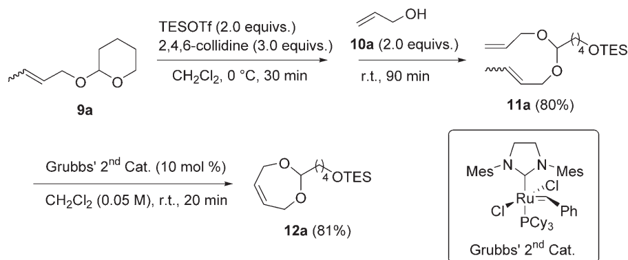
Scheme 7. Formation of mixed acetal 11a , and efficient olefin metathesis.
