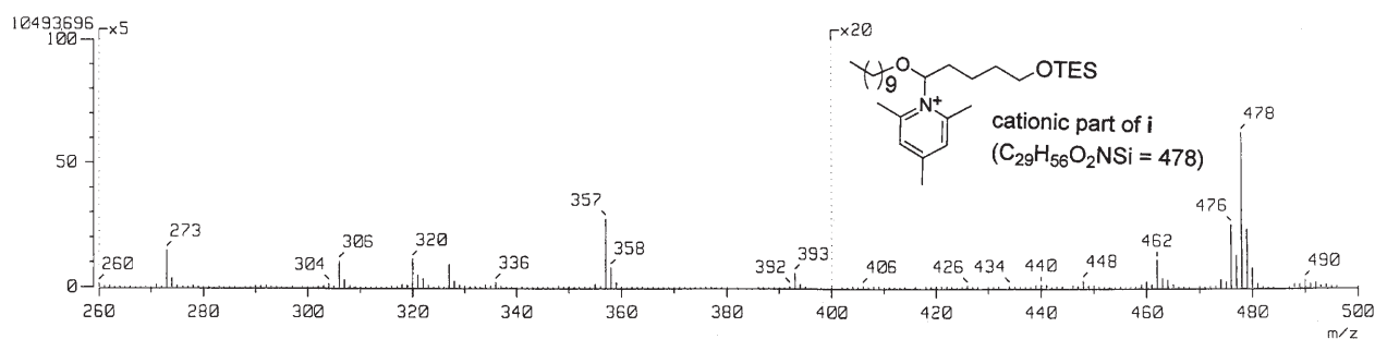
Figure 3. FAB(+)-MS ( m/z = 260\text{--}500 ) of the mixture of 1a , TESOTf, and 2,4,6-collidine.
